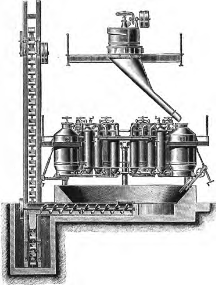
FIG. 15.—SECTIONAL VIEW OF CIRCULAR DIFFUSION BATTERY
